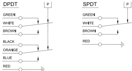
WIRING DIAGRAM FOR CABLE
